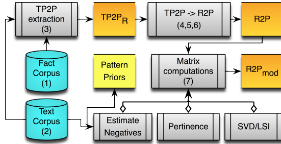
Figure 2: Pattern extraction workflow
