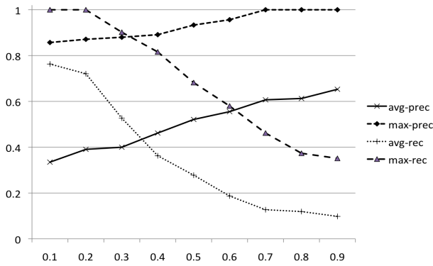
Figure 3: Precision and recall on the DBPedia testing set and the Wikipedia text corpus.
