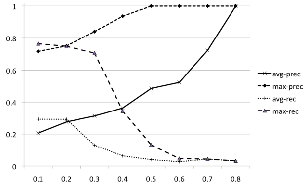
Figure 4: Precision and recall on the UMLS testing set and the MedLine text corpus.
