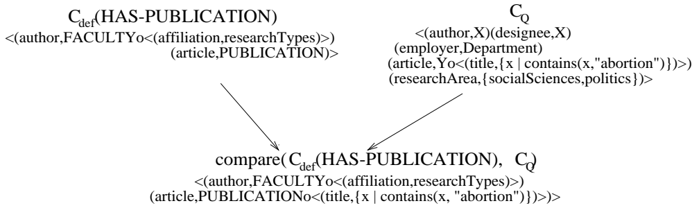
Figure 3: Comparison of contextual descriptions: Incorporating a constraint from the query
