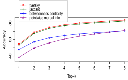
Fig. 2. Top-K accuracy
